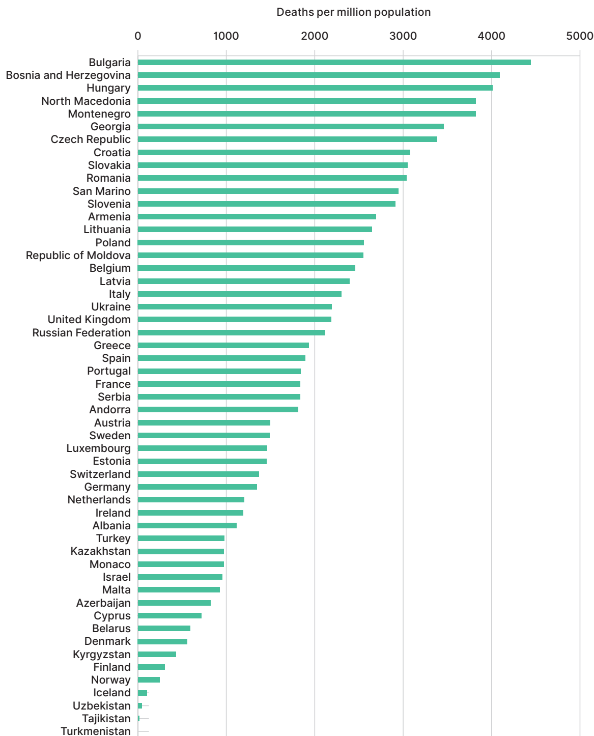
Fig. 3.2. Crude cumulative COVID-19-related mortality rates in the WHO European Region as reported by Member States on 31 December 2021
