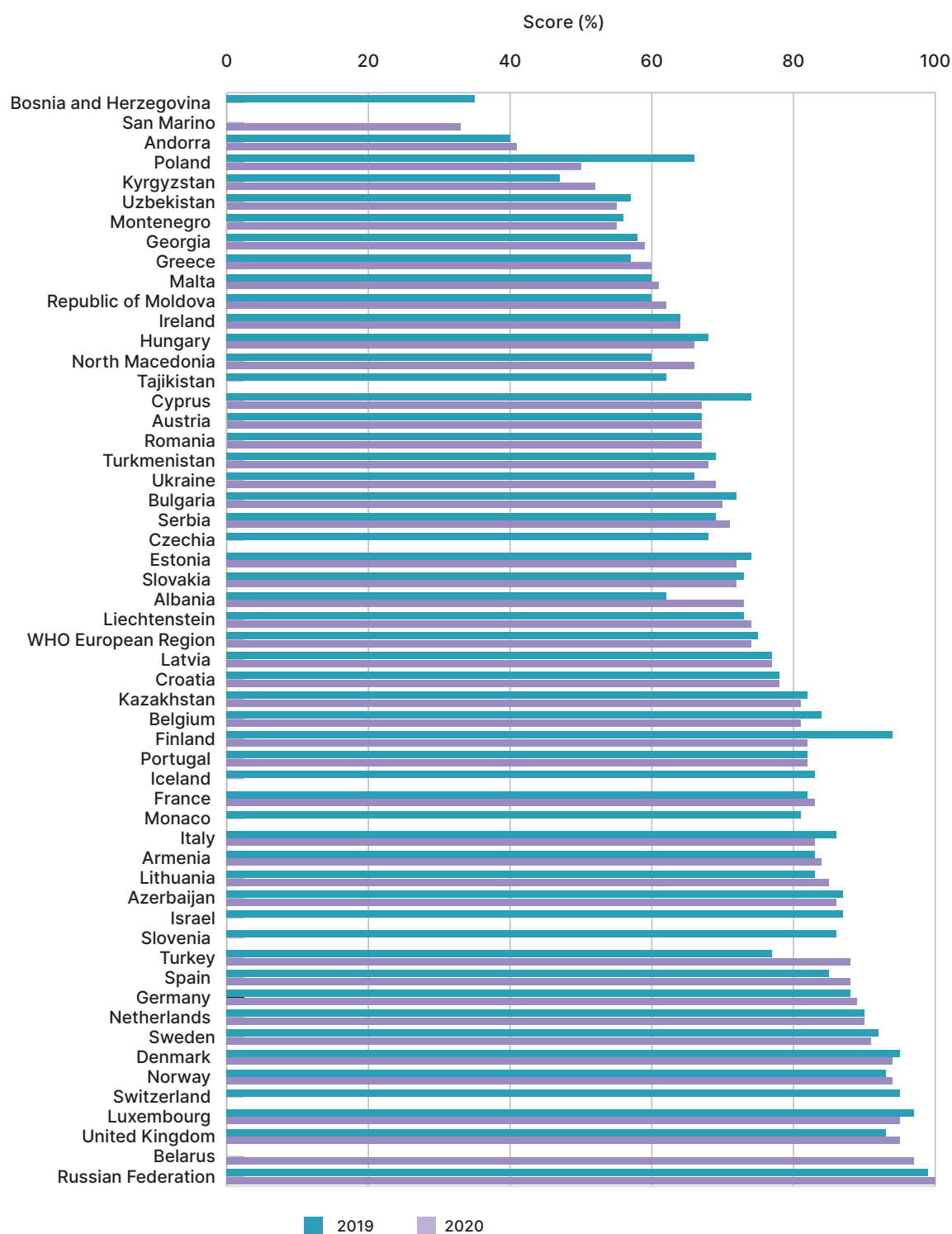
Fig. 2.8. IHR core capacity scores in State Parties of the WHO European Region, 2019 and 2020
