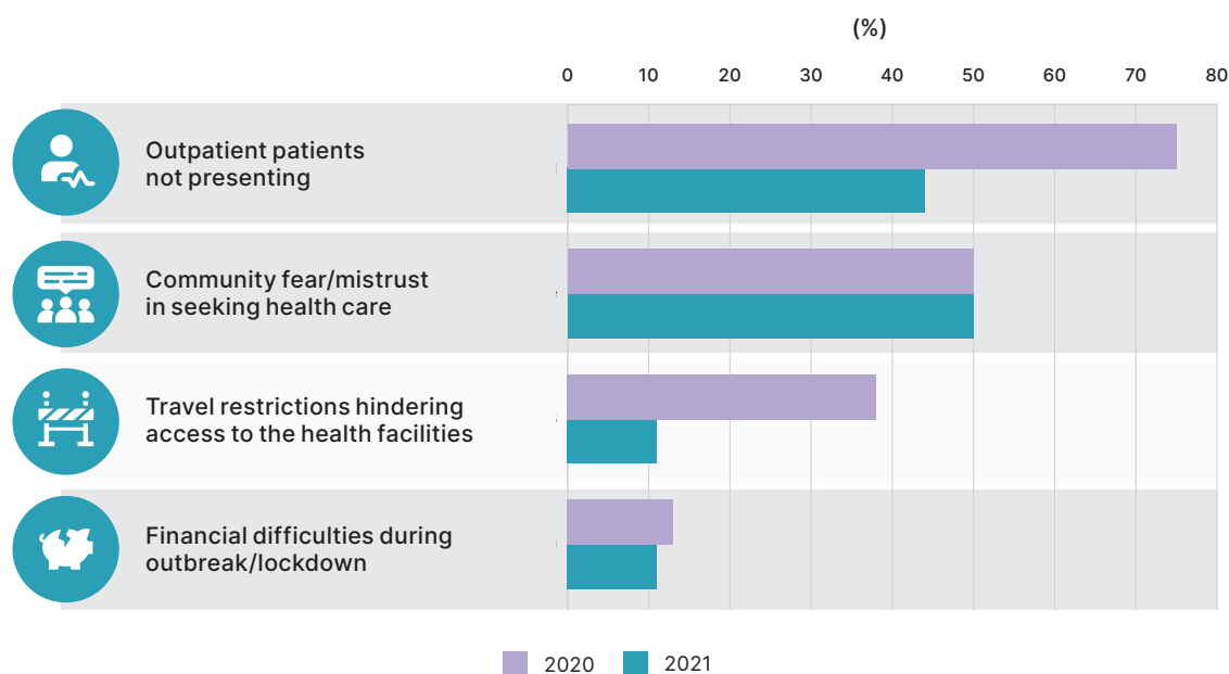
Fig. 3.4. Demand-side reasons reported for service disruption in the WHO European Region
