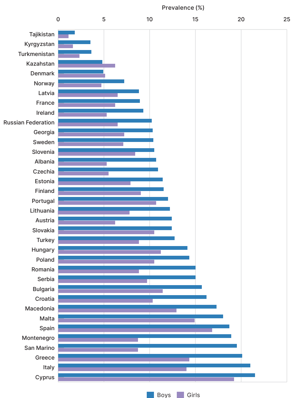
Fig. 2.18. Prevalence of obesity in children aged 7–9 years in Member States of the WHO European Region, 2015–2017
