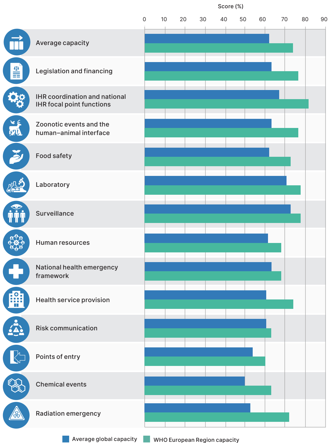
Fig. 2.7. IHR core capacity scores in the WHO European Region and average global capacity, 2020
